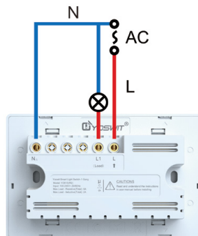
Connection 2: With neutral wire
